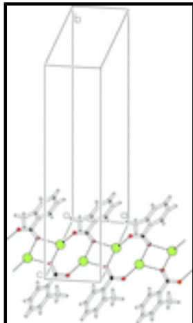
Fig. 2. A partial packing diagram ( PLATON ; Spek, 2009) which shows that the molecules are interlinked to form polymeric chains.
